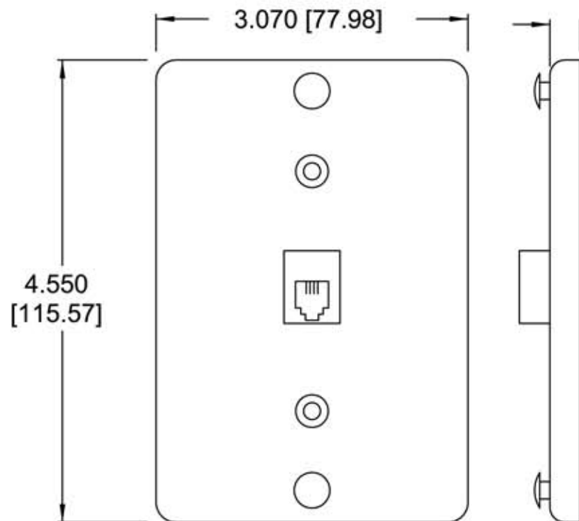
STAINLESS STEEL COVER
